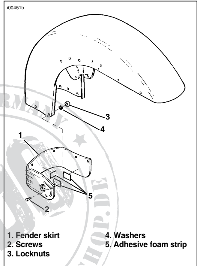
Front Fender Skirt and Assembling Hardware
