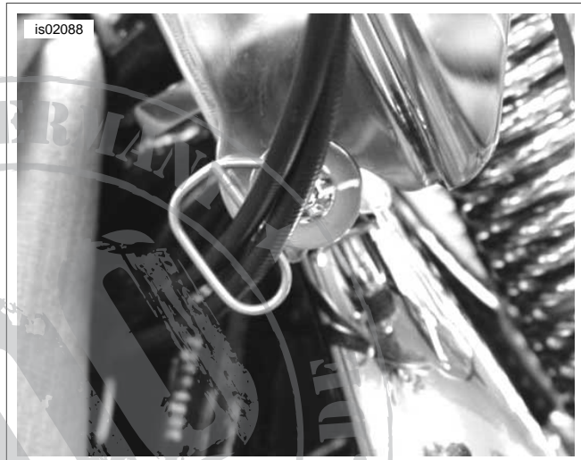
Figure 2. Throttle Cable Guide (All Models Except FLSTSB, FXSTSSE and FXSTSSE2)
