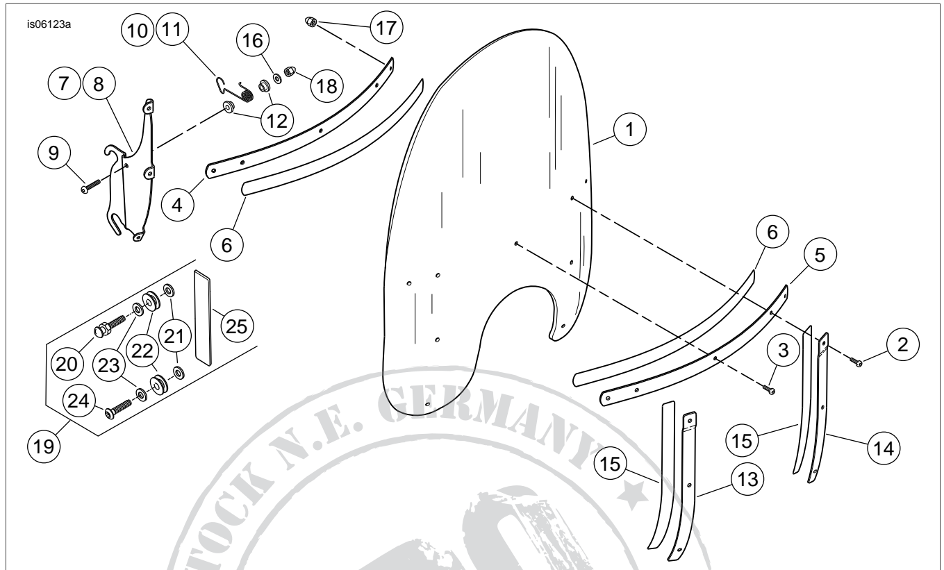
Figure 2. Service Parts for Windshield Kit
