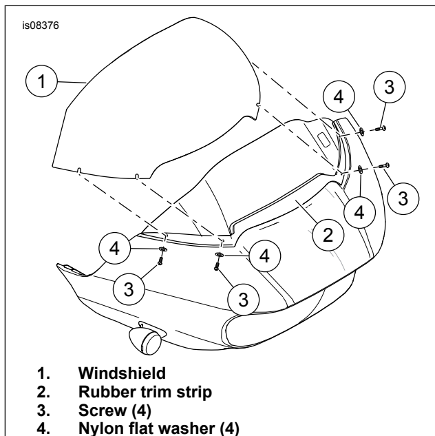
Figure 1. Windshield Installation
