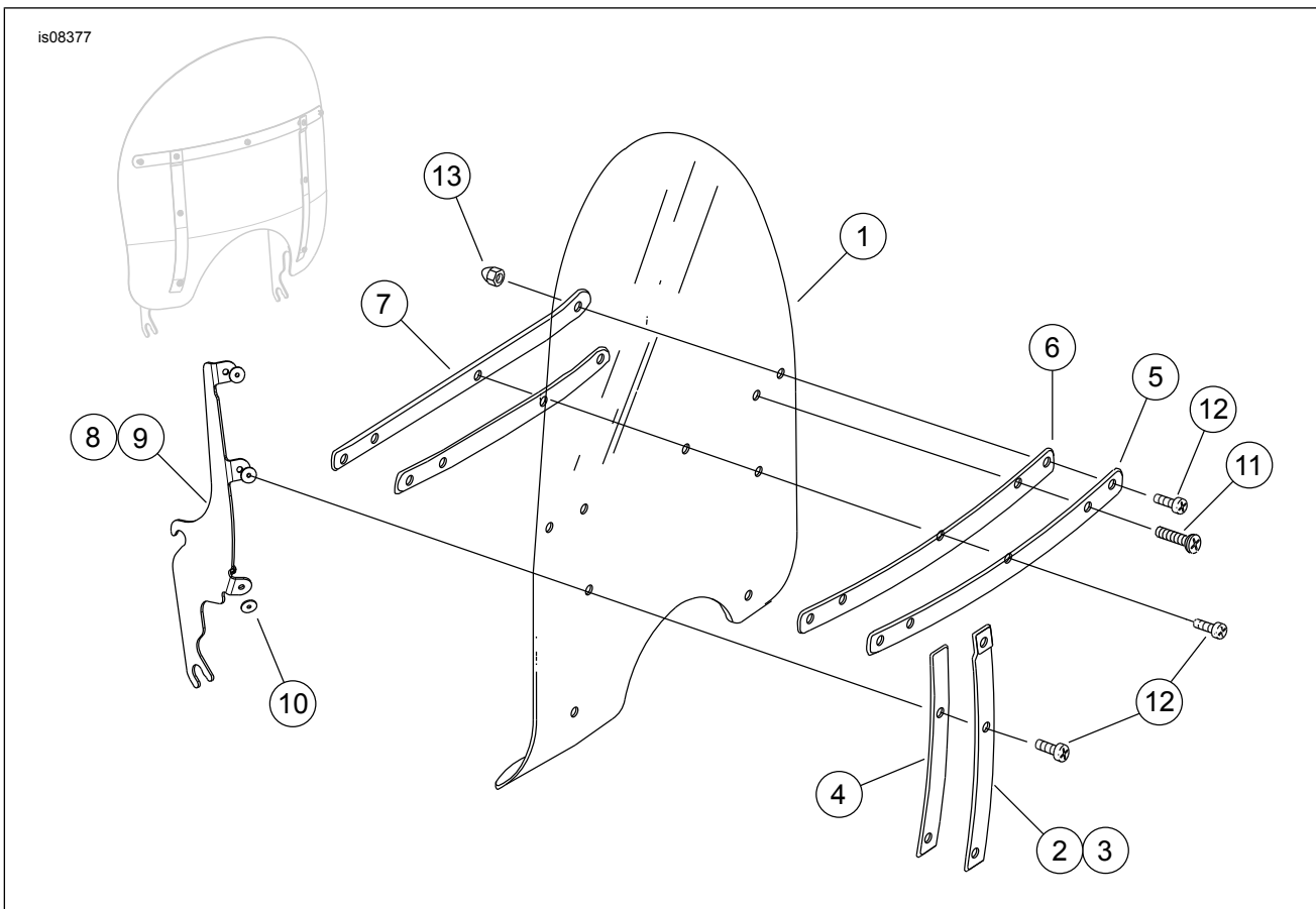
Figure 1. Service Parts
