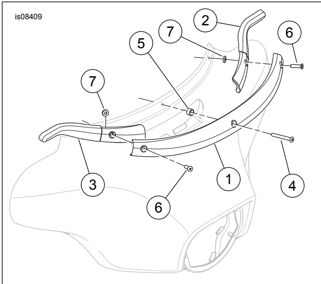
Figure 2. Service Parts, Windshield Trim Mirror Mount Kit
