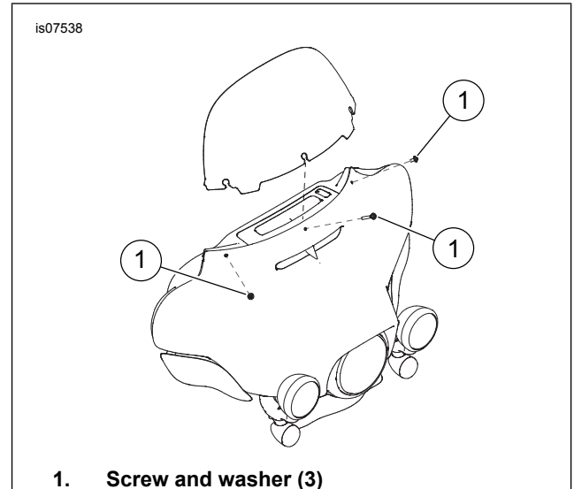
Figure 1. Windshield Installation
