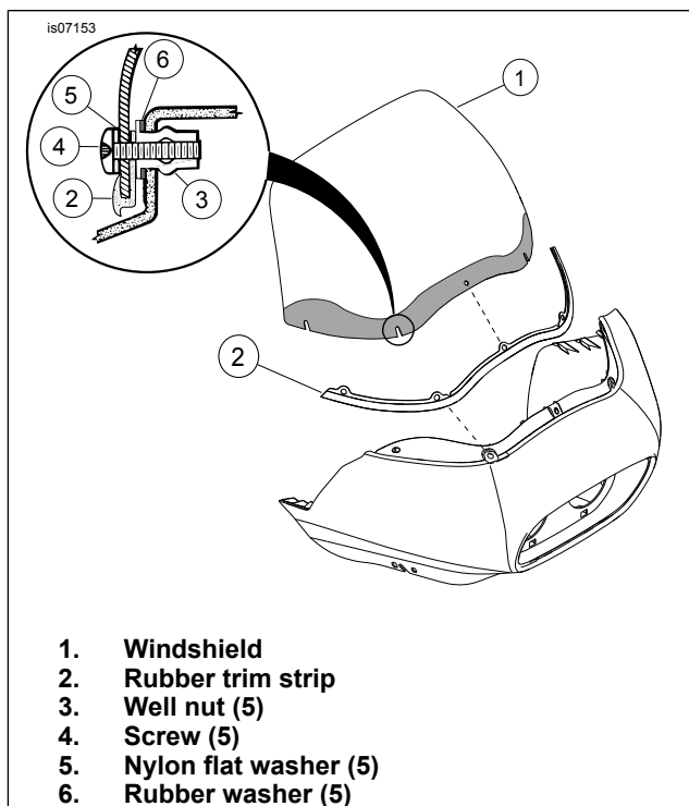
Figure 1. Windshield Installation
