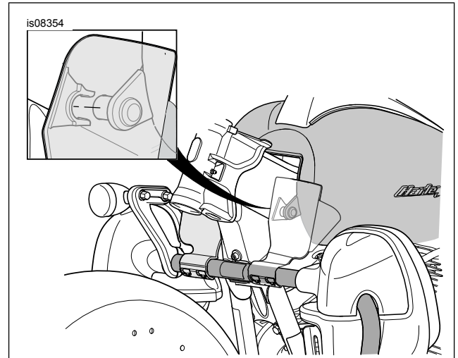
Figure 1. Air Deflector
