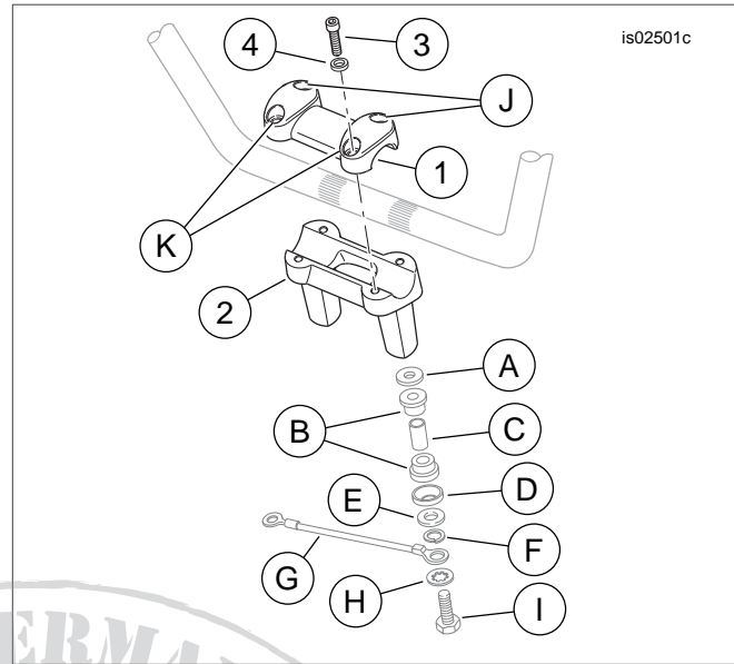
Figure 1. Service Parts, One-Piece Fat Handlebar Riser Kits
