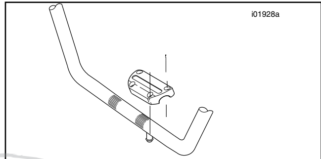
Figure 1. Install new handlebar clamp with existing hardware
