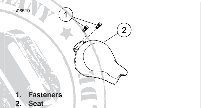
Figure 1. Solo Seat
