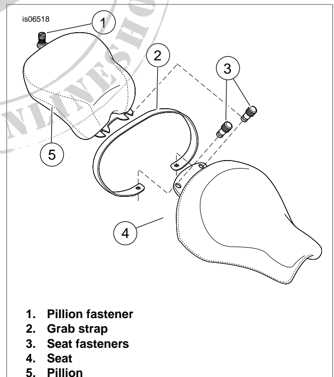
Figure 2. 2-Up Seat
