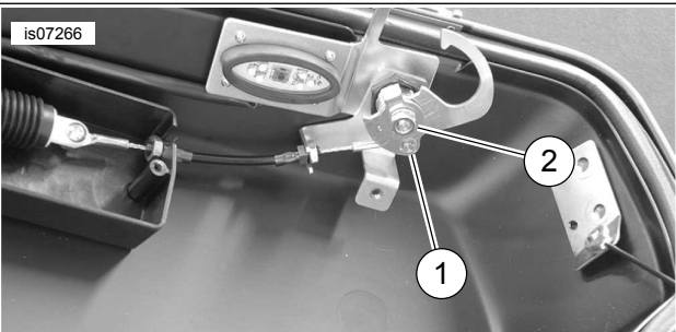
Figure 3. Tour-Pak Latch Cover
