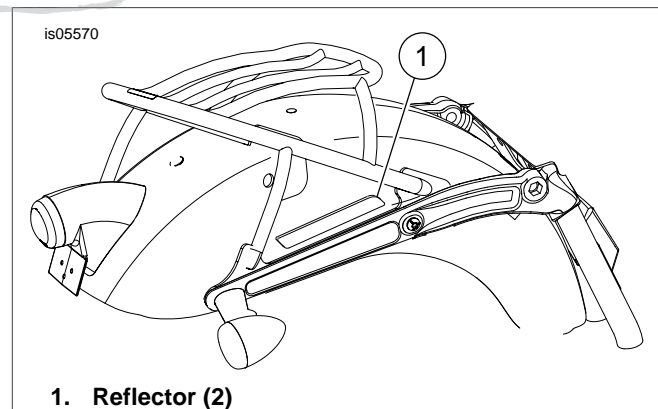
Figure 4. Install Reflector
