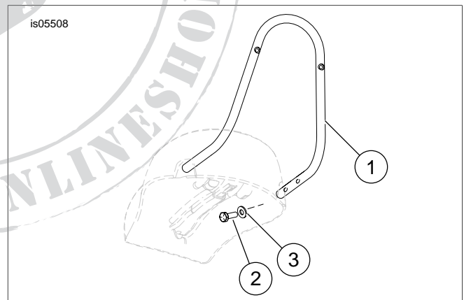
Figure 2. Service Parts: Passenger Pillion Upright
