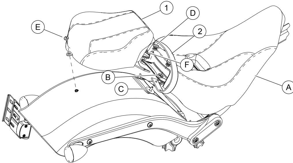
Figure 1. Service Parts: Detachable Pillion Seat
