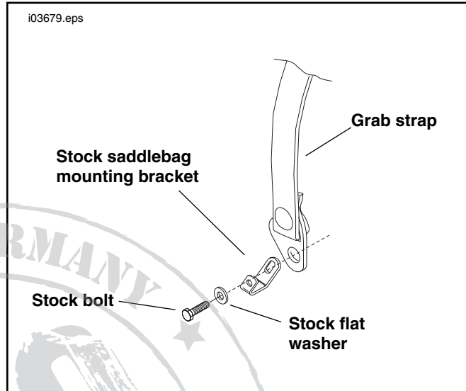
Figure 1. Vehicle Grab Strap Mounting Orientation
