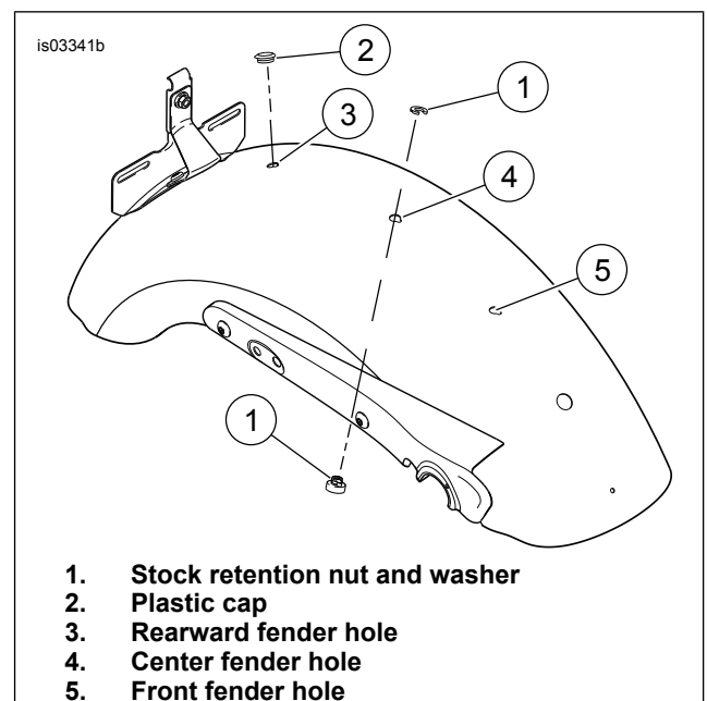
Figure 1. Retention Nut and Plastic Cap Location
