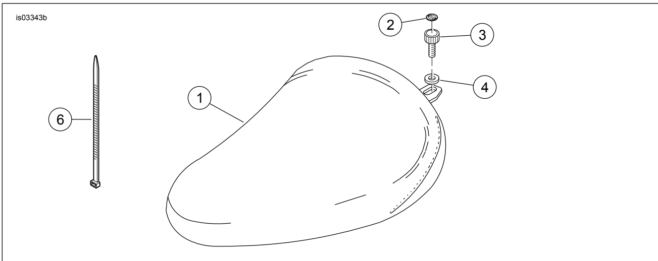
Figure 3. Service Parts for XL Solo Custom Seat Kits
