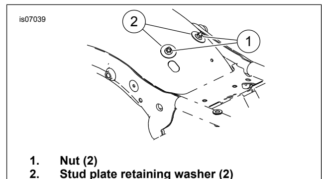
Figure 2. Nuts and Stud plate washers
