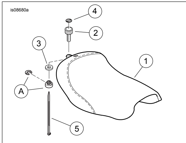
Figure 4. Service Parts: Dyna Solo Seat Kit
