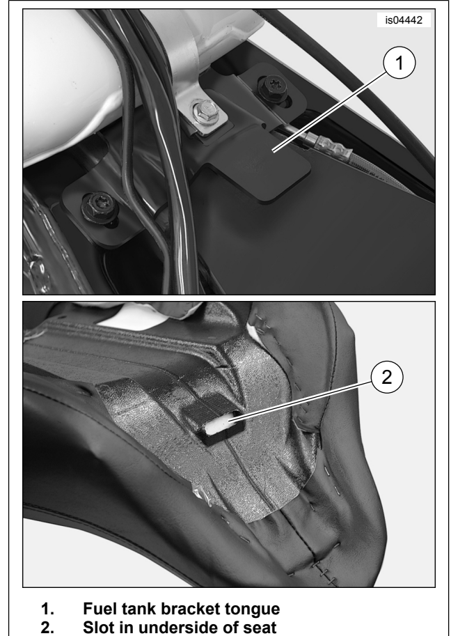
Figure 1. Seat Front Mounting
