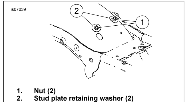
Figure 1. Remove Nuts
