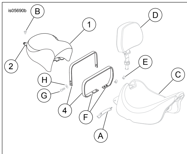
Figure 2. Service Parts: Pillion Kit
