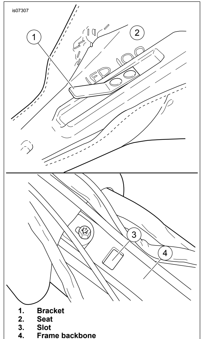
Figure 2. Seat Bracket and Mounting Slot
