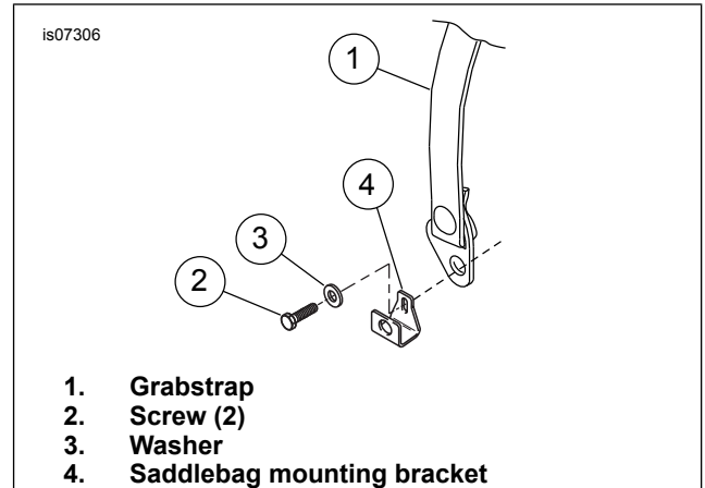
Figure 1. Grabstrap Mounting Orientation
