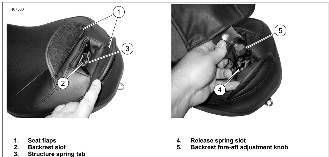
Figure 3. Backrest
