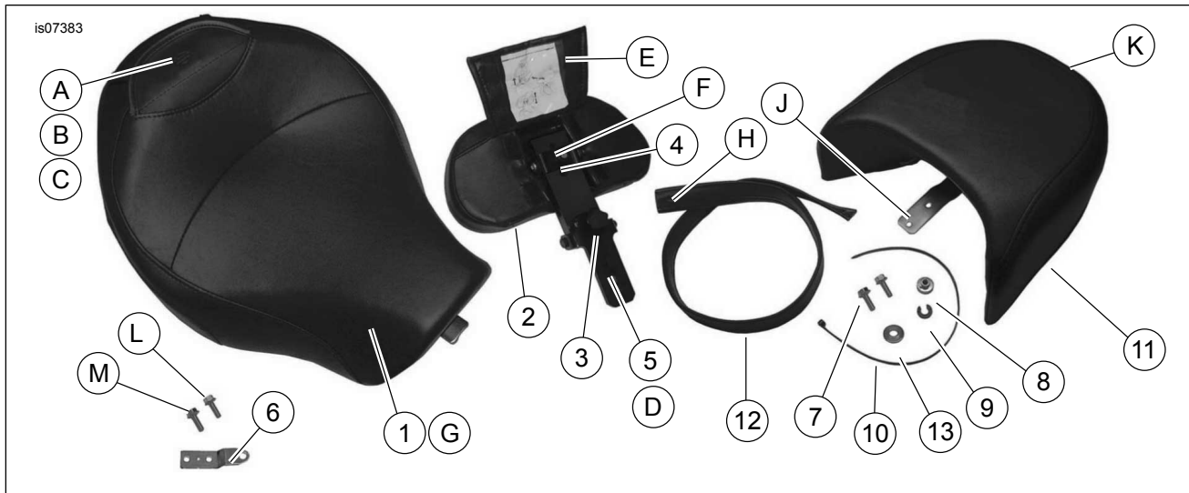
Figure 4. Service Parts
