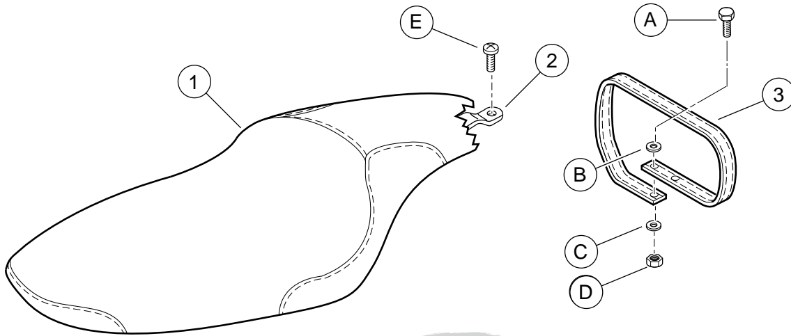
Figure 2. Service Parts: Softail Seats
