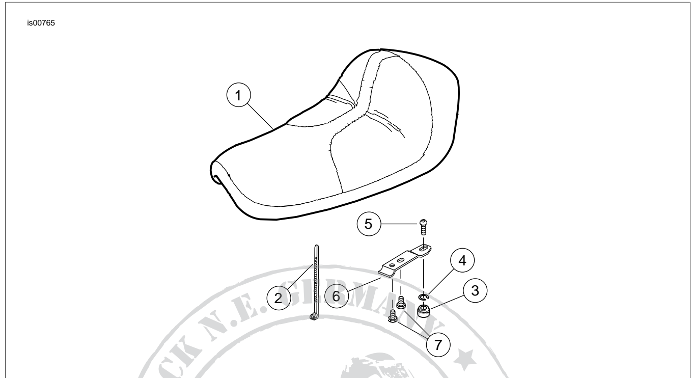
Figure 3. Service Parts: Dyna Solo Seat
