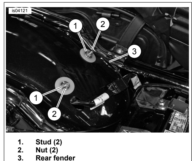
Figure 1. Rear Fender
