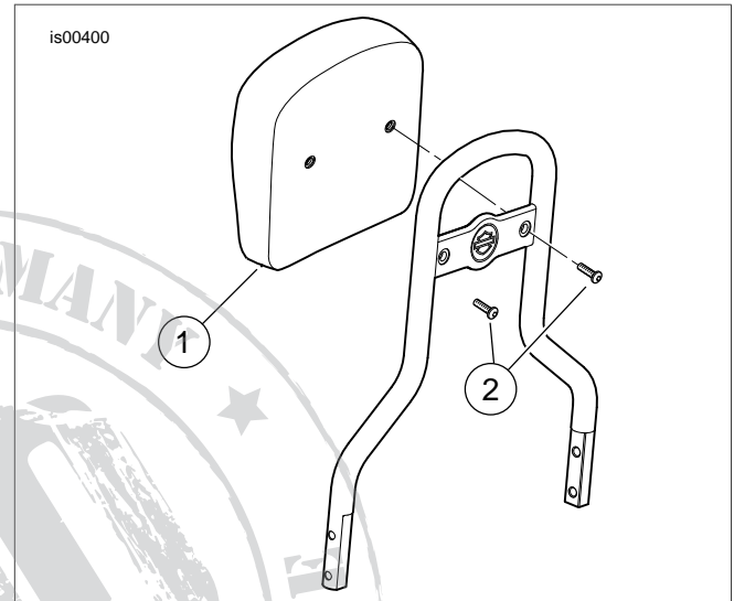
Figure 1. Service Parts: FL Backrest Pad Kits
