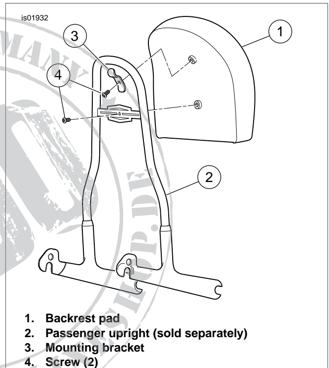
Figure 1. Passenger Backrest
