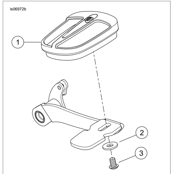
Figure 1. Slipstream Brake Pedal Kit Contents
