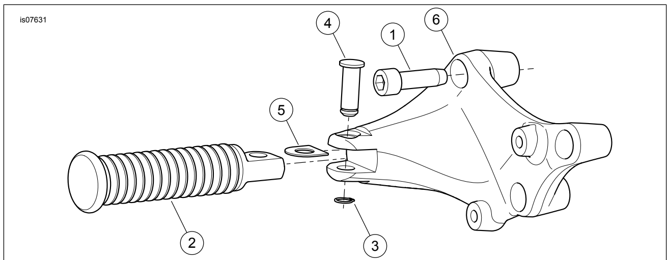
Figure 1. Service Parts: Passenger Footpeg Mounting Kit
