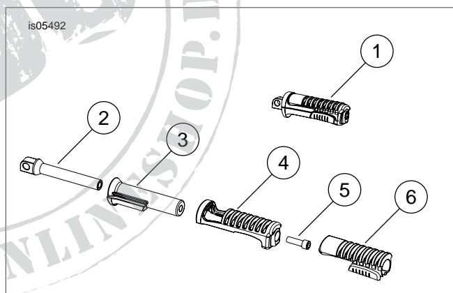
Figure 2. Service Parts: X2 Footpeg Kit
