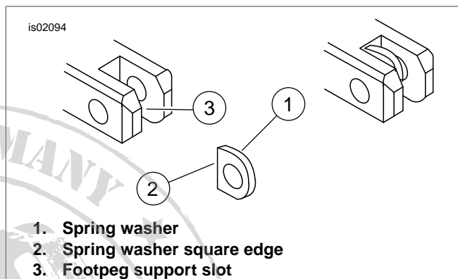
Figure 1. Footpeg Spring Washer Installation
