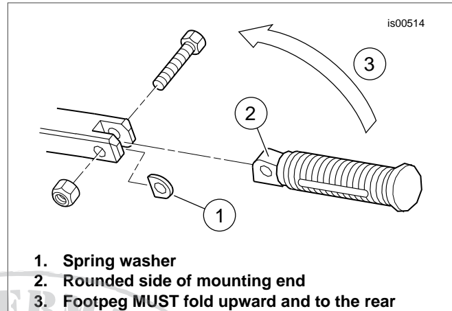
Figure 4. Proper Footpeg Installation
