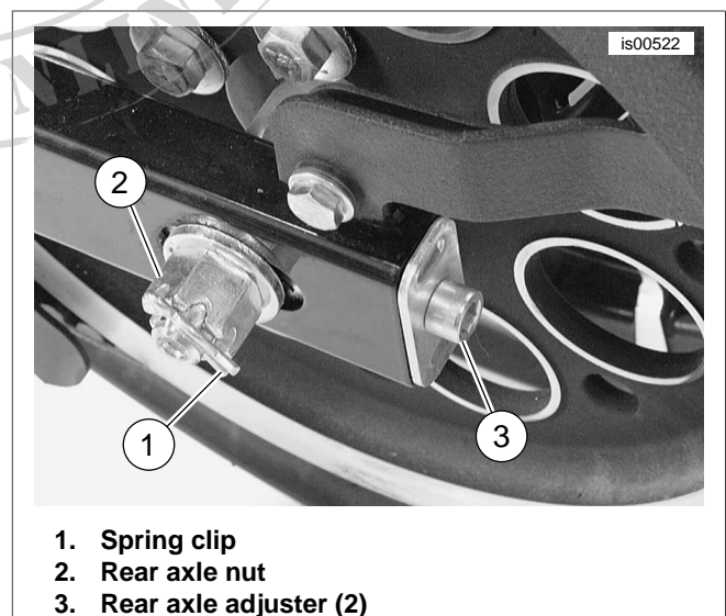
Figure 2. Rear Axle Nut and Adjusters
