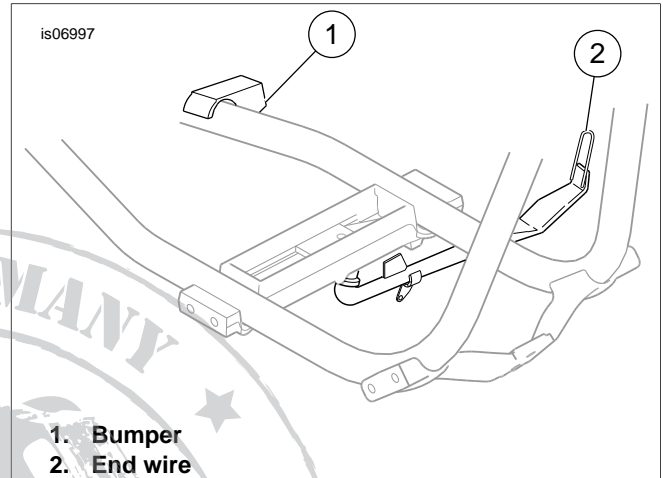
Figure 1. End Wire and Bumper
