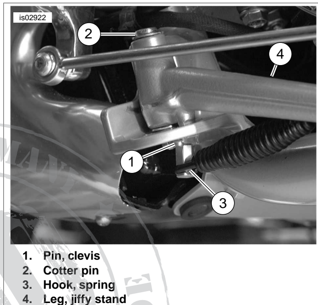
Figure 1. Jiffy Stand Components
