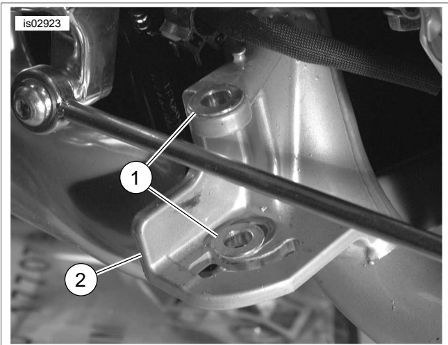
Figure 2. Jiffy Stand Mounting Bracket
