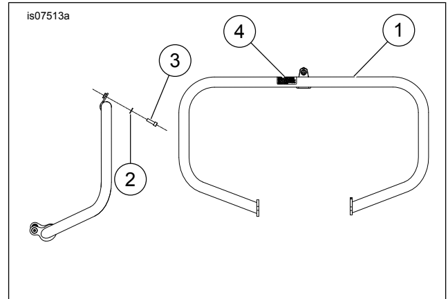
Figure 1. Service Parts: Engine Guard Kit
