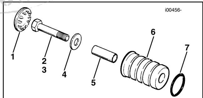
Figure 1. Exploded view
