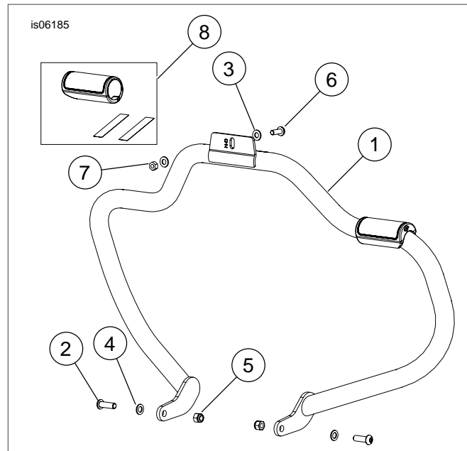
Figure 4. Service Parts: Mustache Engine Guard
