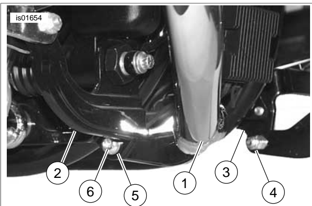
Figure 2. Engine Guard Mounting Flange (Top Center)
