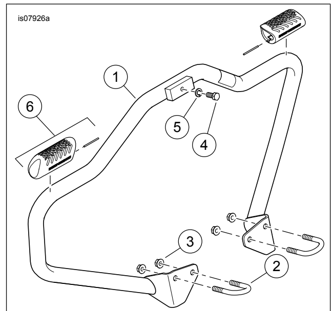
Figure 2. Service Parts: Dyna Engine Guard Kit
