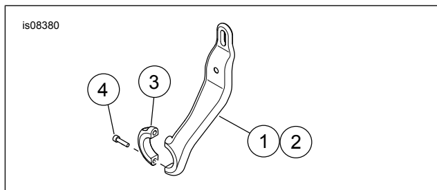
Figure 1. Service Parts: Support Bracket
