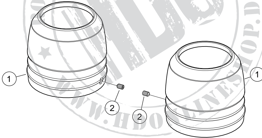
Figure 3. Service Parts, Fork Slider Dust Cover Kit
