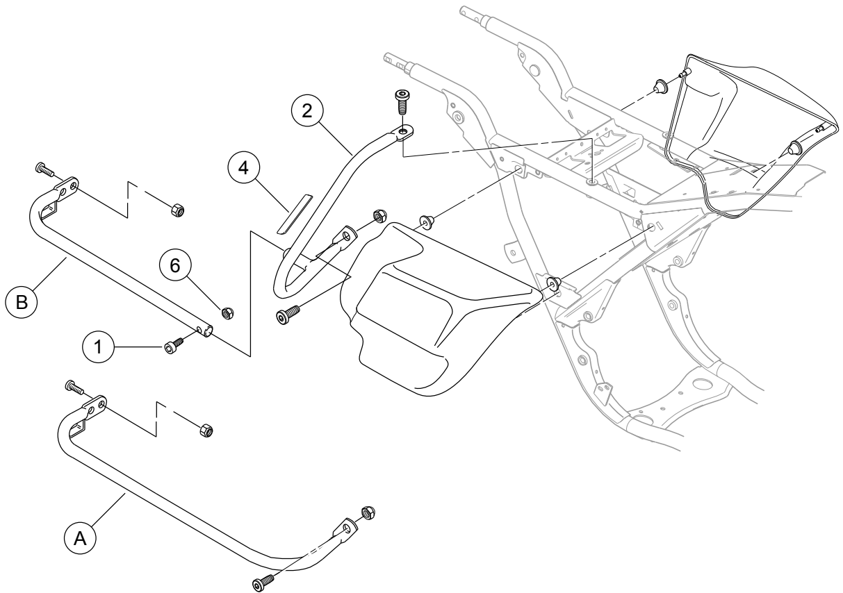
Figure 2. Service Parts: Rear Saddlebag Guard Kit (Black)
