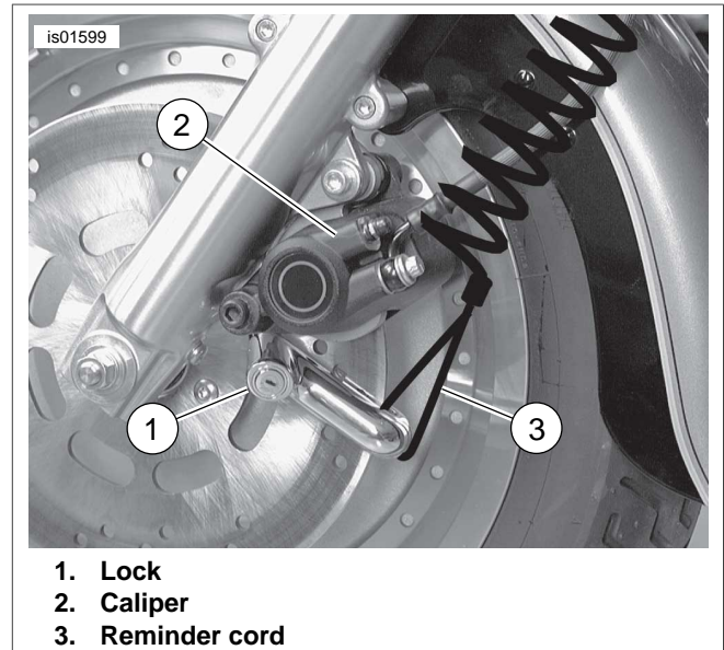
Figure 1. Installing Disc Lock
