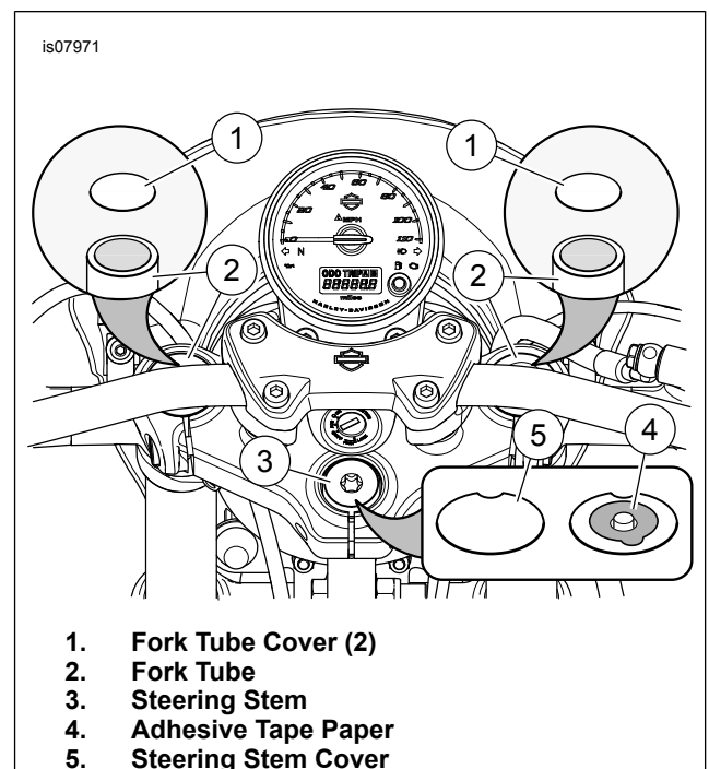
Figure 1. Fork Tube and Steering Stem Covers
