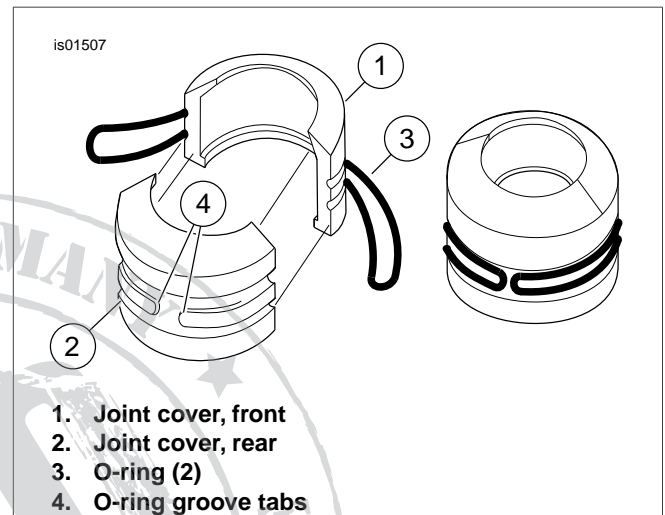
Figure 1. Fork Joint Cover
