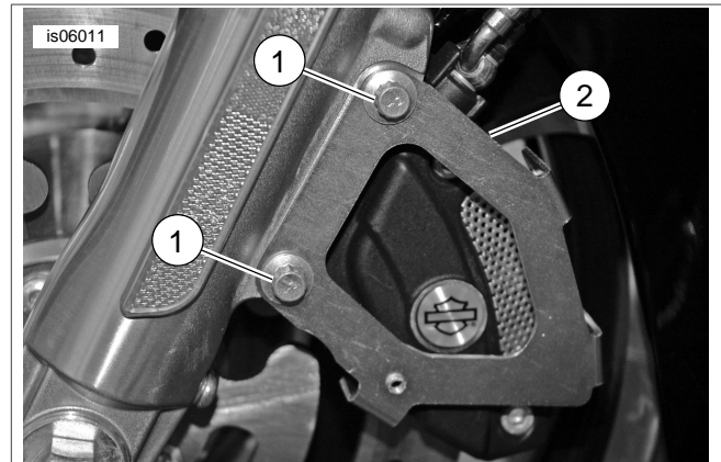
Figure 1. Install Caliper Mounting Bracket
