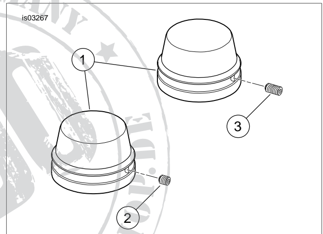
Figure 1. Front Axle Nut Covers
