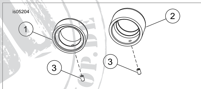
Figure 1. Rear Axle Nut Cover Kit
