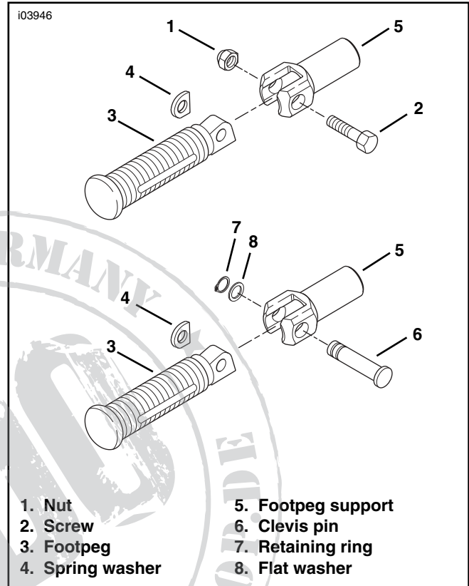
Figure 1. Footpeg Mounting Pins
